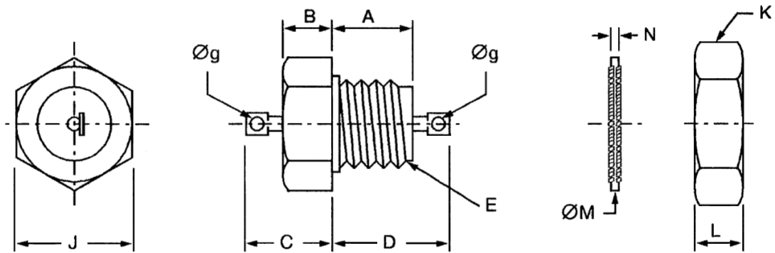
FIGURE 2 – PHYSICAL DIMENSIONS
