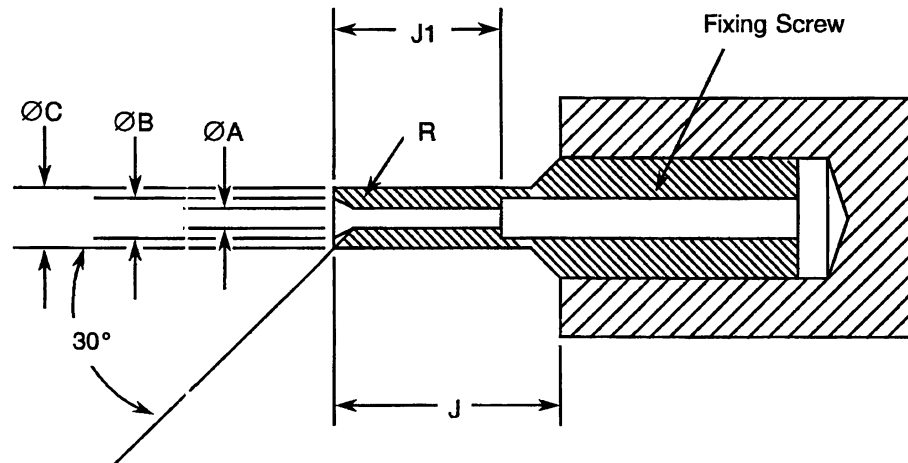
MAXIMUM GAUGE
