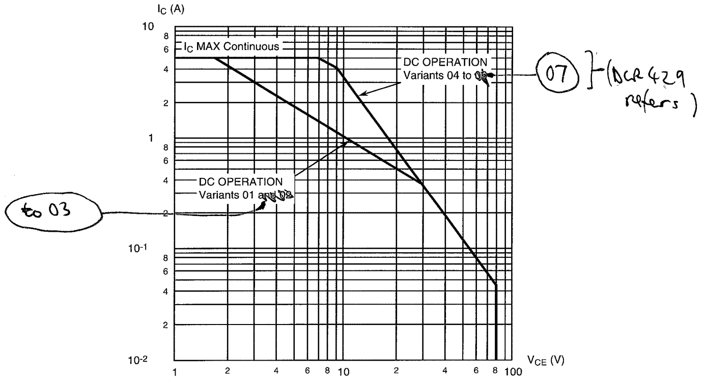
Maximum Safe Operating Area Graph
