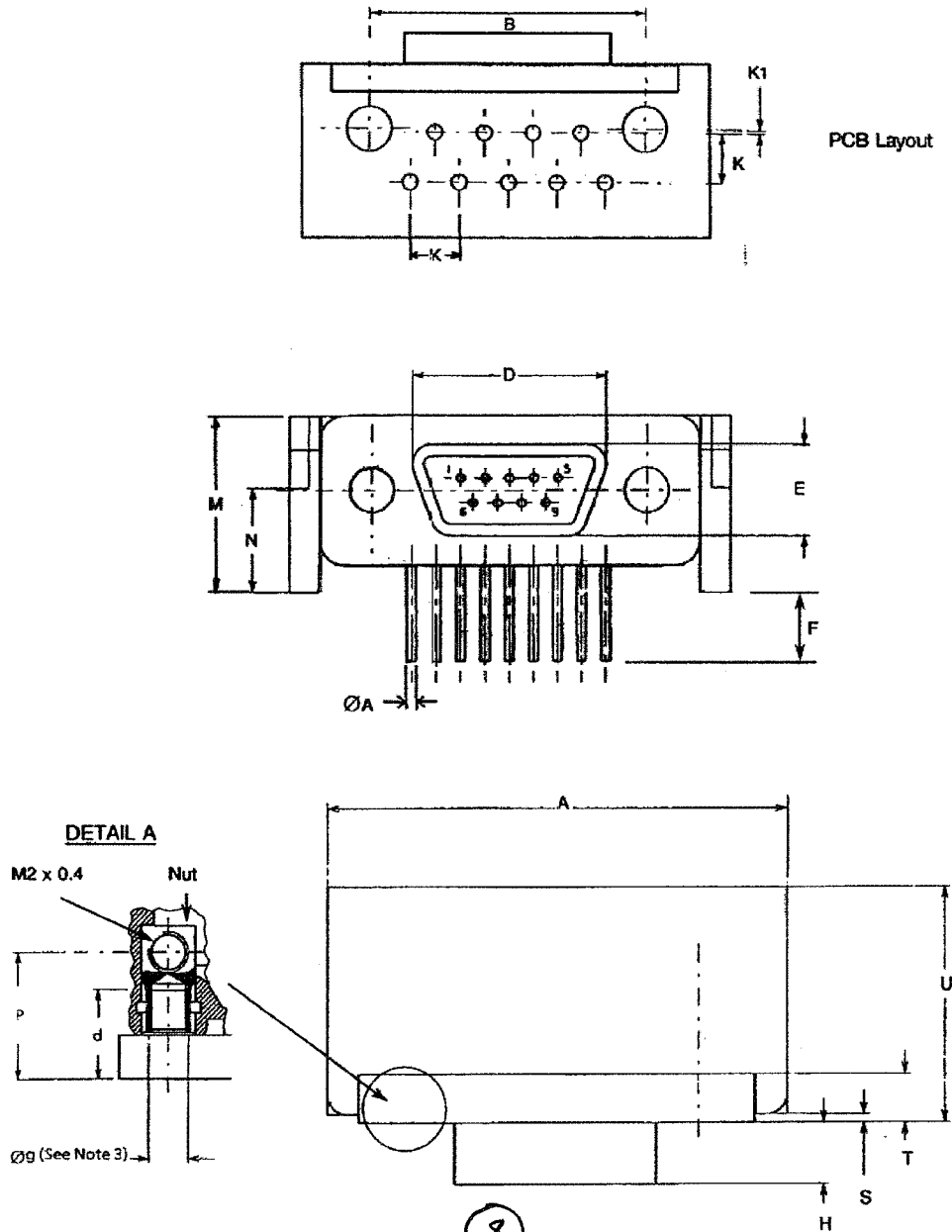
FIGURE 2.2F - CONNECTORS TYPE - FR136A RECEPTACLE FEMALE CONTACTS
