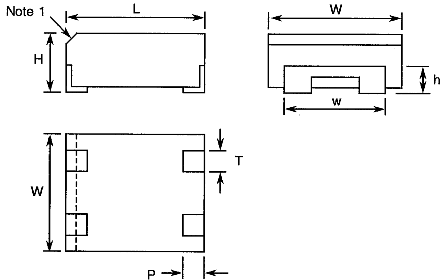
FIGURE 2 - PHYSICAL DIMENSIONS
