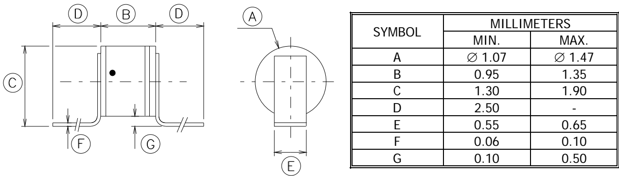
FIGURE 2(a) – Variants 01, 08, 15, 22, 29, 36, 43
