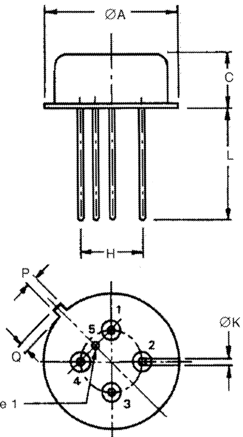
FIGURE 2 - PHYSICAL DIMENSIONS
