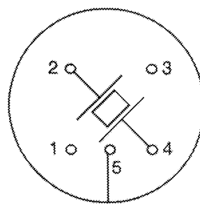
FIGURE 3 - FUNCTIONAL DIAGRAM
