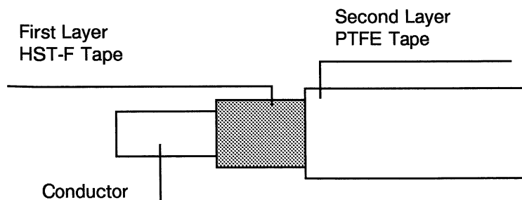
FIGURE 2(a) - FINISHED WIRES
