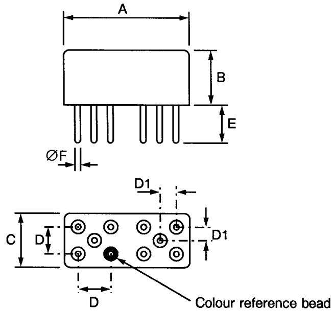
FIGURE 2(j) - VARIANT 01, RELAY WITH LONG PLUG-IN TERMINALS AND PLAIN CASE
