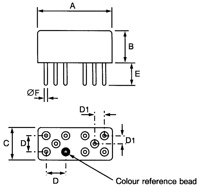
FIGURE 2(i) - VARIANT 09, RELAY WITH LONG PLUG-IN TERMINALS AND PLAIN CASE
