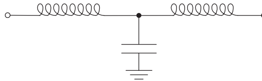
FIGURE 3 - FUNCTIONAL DIAGRAM
