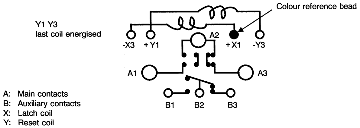
FIGURE 3 - CIRCUIT SCHEMATIC
