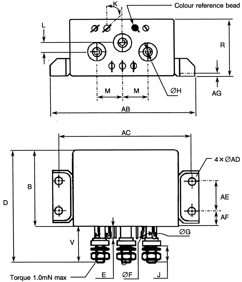
FIGURE 2(b) - VARIANT 04 - RELAY WITH SIDE FLANGE
