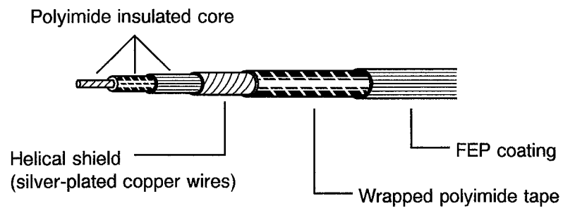
FIGURE 2(b) - SHIELDED AND JACKETED CABLES
