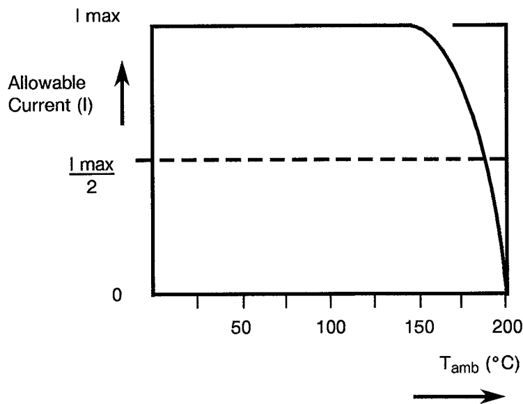
Allowable Current versus Temperature
