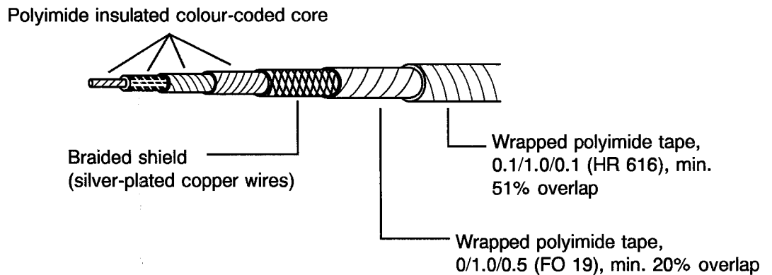
FIGURE 2(b) - SHIELDED AND JACKETED CABLES
