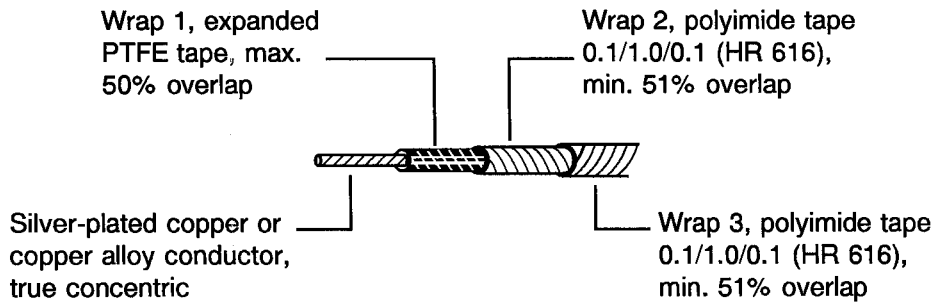
FIGURE 2(a) - FINISHED WIRES
