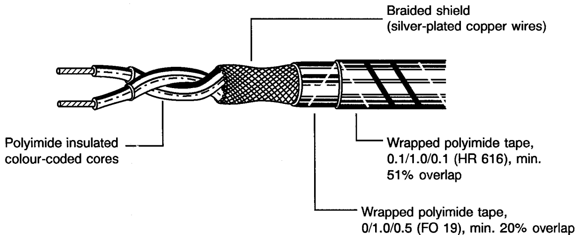
FIGURE 2(c) - SHIELDED AND JACKETED CABLES
