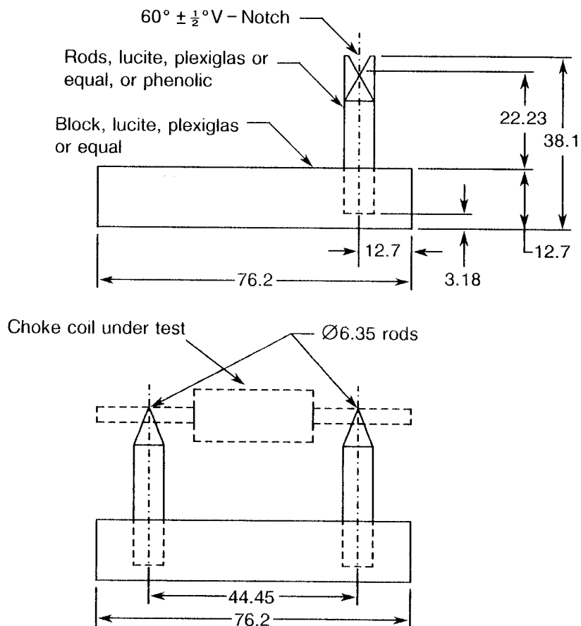
FIGURE VI - TEST FIXTURE FOR SELF-RESONANT FREQUENCY TEST (FOR AXIAL LEADS)
