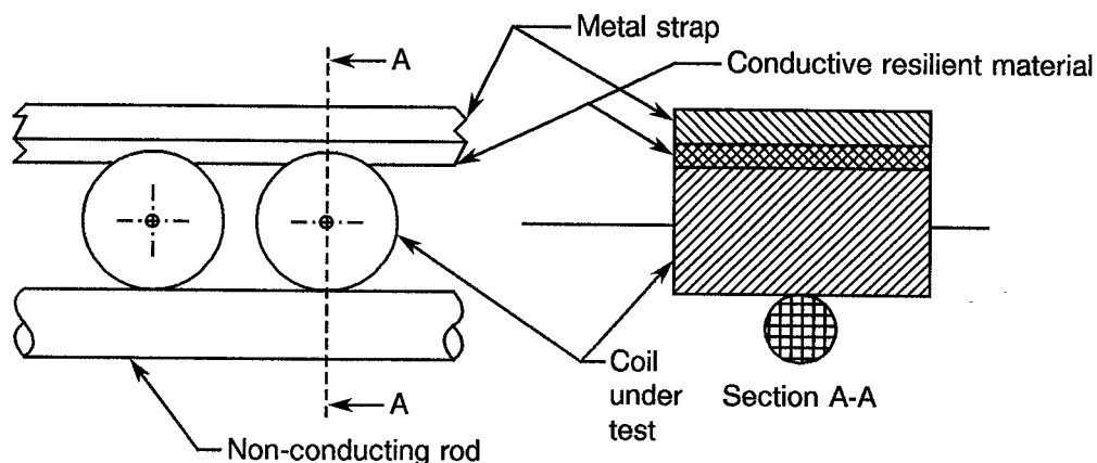
FIGURE VIII - COIL-CONTACTING ASSEMBLY FOR MOUNTING DURING POLARISATION
