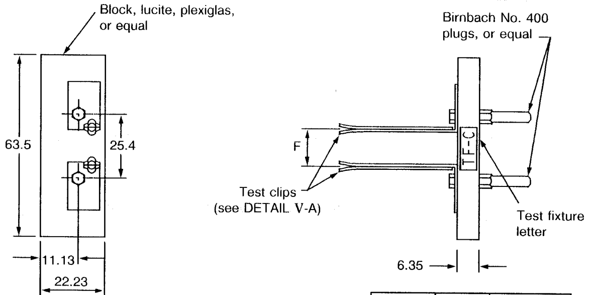
FIGURE V - TEST FIXTURE TF-C, TF-D AND TF-E (FOR RADIAL LEADS)
