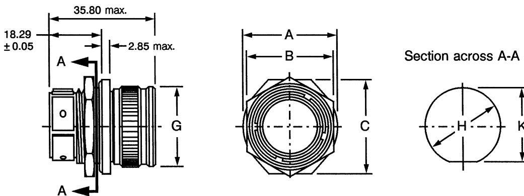
SHELL TYPE 74 - SINGLE HOLE MOUNTING RECEPTACLE
