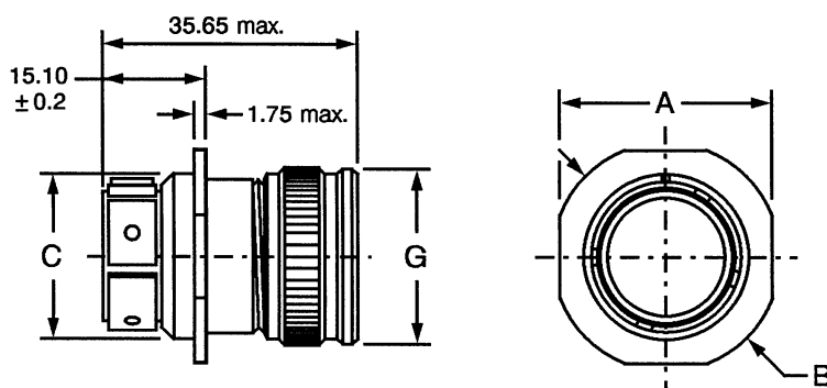
SHELL TYPE 71 - CABLE CONNECTING RECEPTACLE
