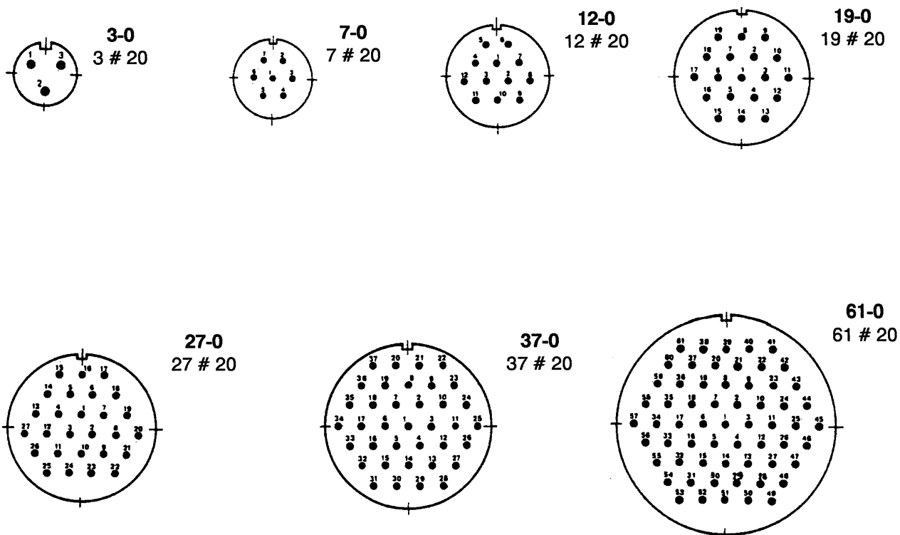
FIGURE 2(a) - STANDARD CONTACT ARRANGEMENTS - FRONT VIEW MALE INSERT (See Para. 4.5 for definition of numbers)
