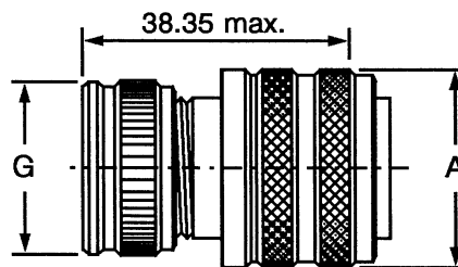
SHELL TYPE 76 - PLUG
