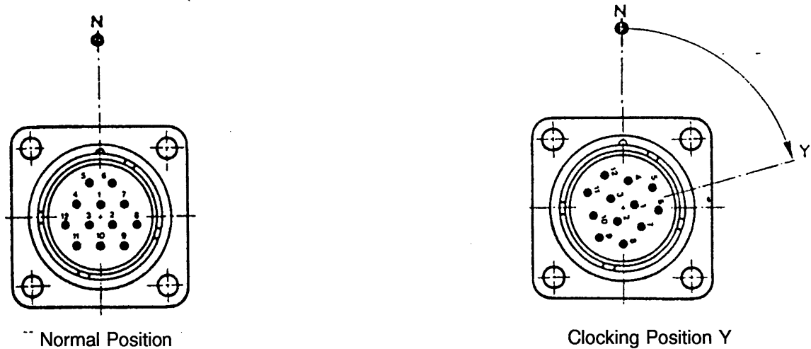
FIGURE 2(c) - INSERT CLOCKING POSITIONS
