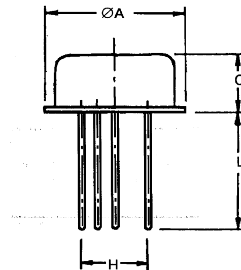
FIGURE 2 - PHYSICAL DIMENSIONS
