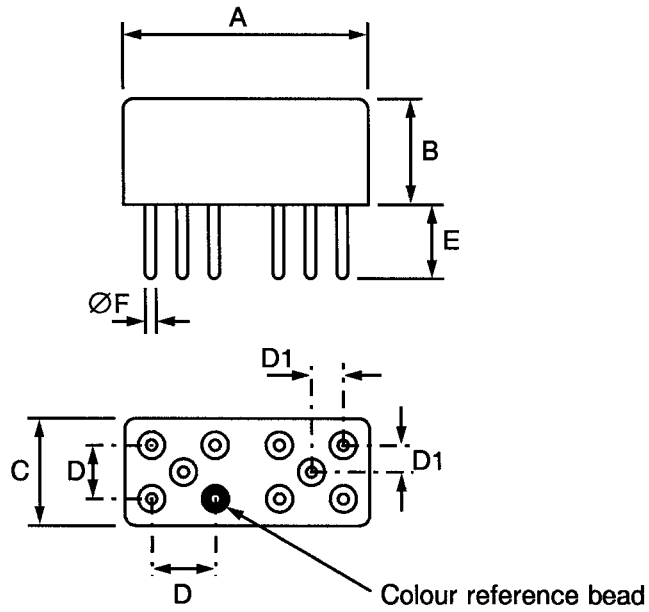
FIGURE 2(i) - VARIANT 09, RELAY WITH PLUG-IN TERMINALS AND PLAIN CASE
