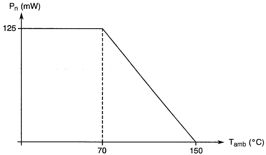
Rated Dissipation versus Temperature
