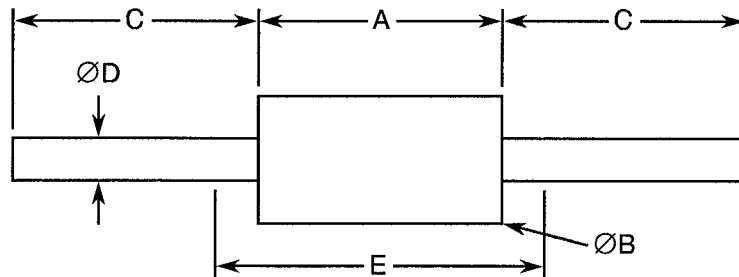
FIGURE 2 - PHYSICAL DIMENSIONS
