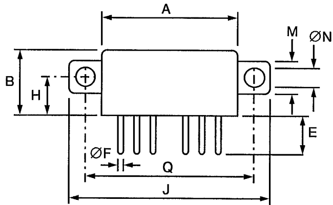
FIGURE 2(d) - VARIANT 04, RELAY WITH PLUG-IN TERMINALS AND VERTICAL SHOULDER BRACKETS
