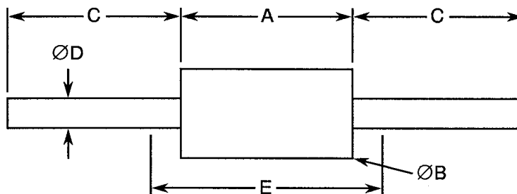
FIGURE 2 - PHYSICAL DIMENSIONS
