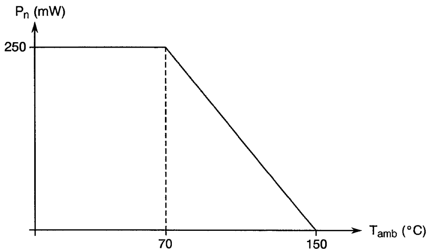
Rated Dissipation versus Temperature
