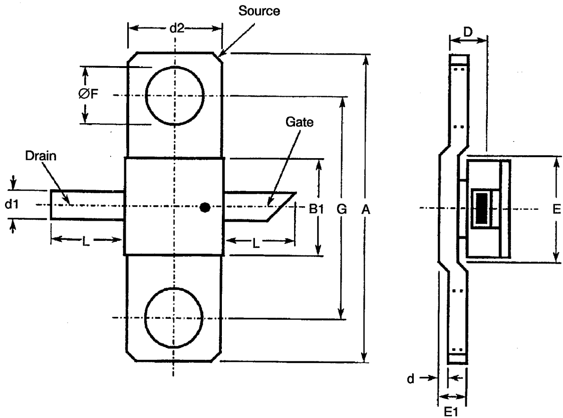
FIGURE 2 - PHYSICAL DIMENSIONS
