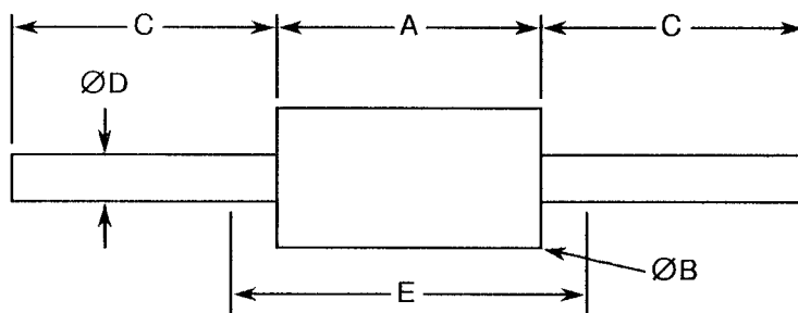
FIGURE 2 - PHYSICAL DIMENSIONS
