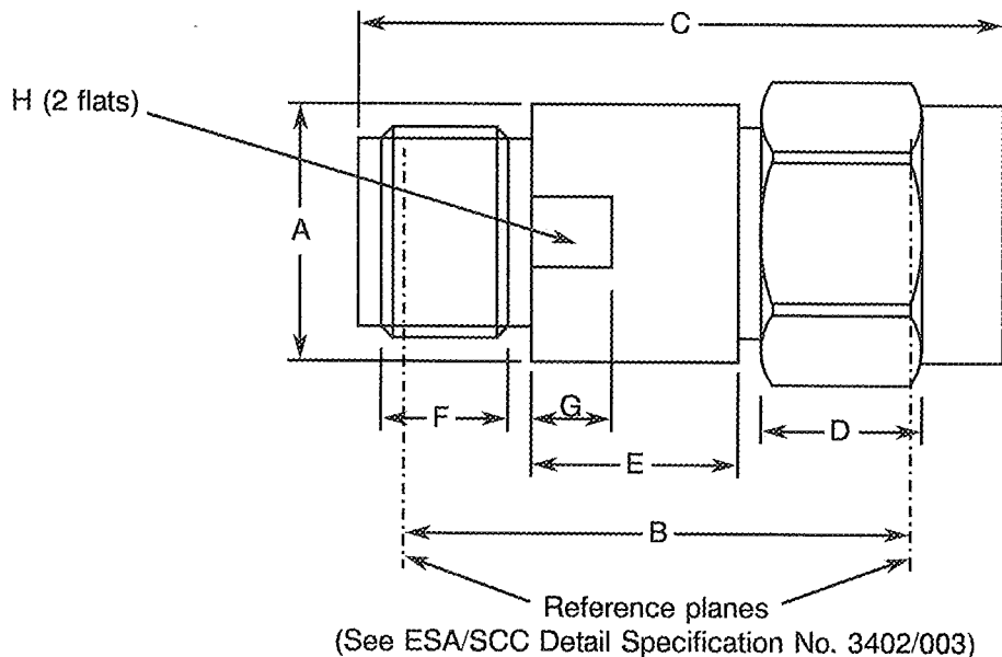
FIGURE 2 - PHYSICAL DIMENSIONS
