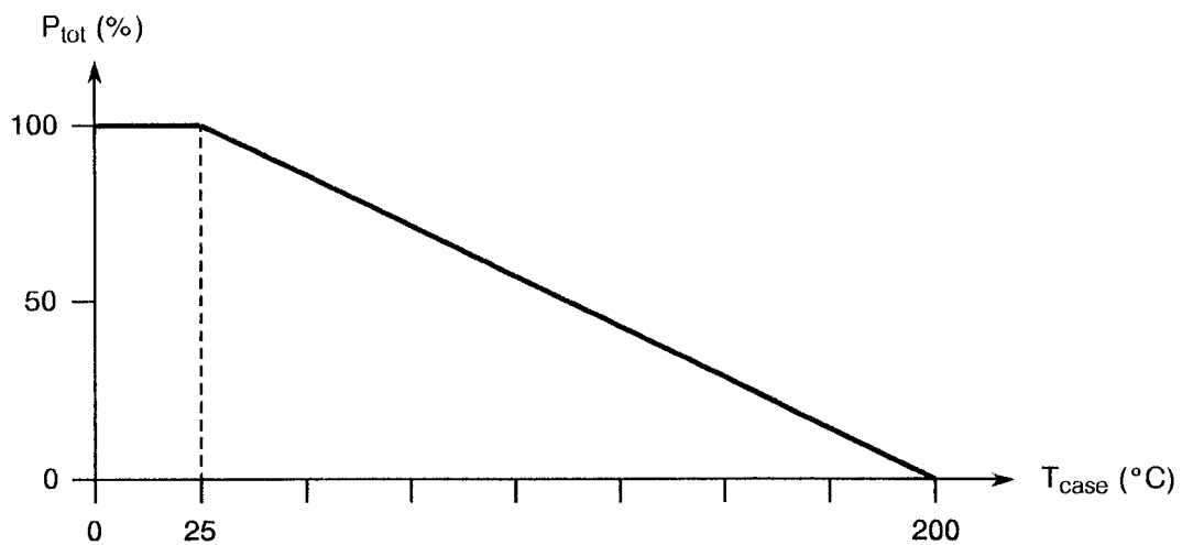
Power Dissipation versus Temperature
