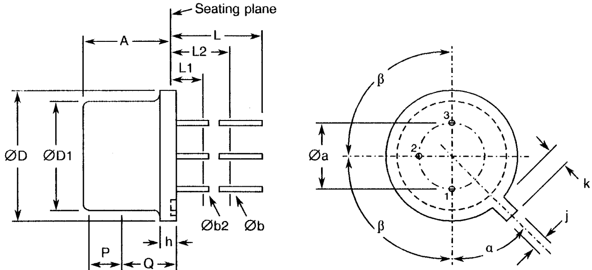
FIGURE 2 - PHYSICAL DIMENSIONS
