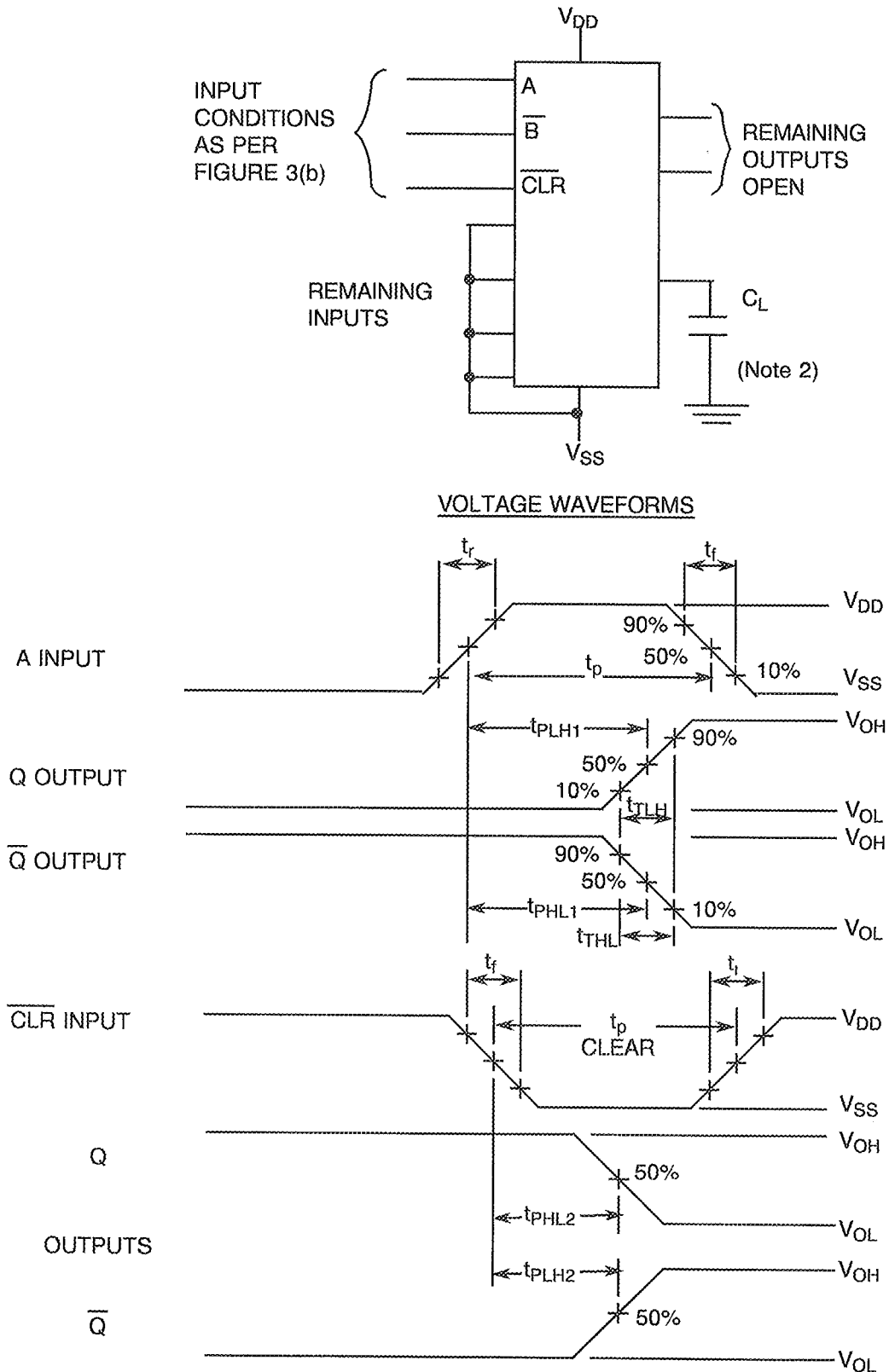
FIGURE 4(i) - PROPAGATION DELAY AND TRANSITION TIME
