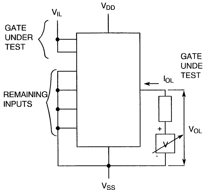
FIGURE 4(d) - OUTPUT VOLTAGE LOW LEVEL
