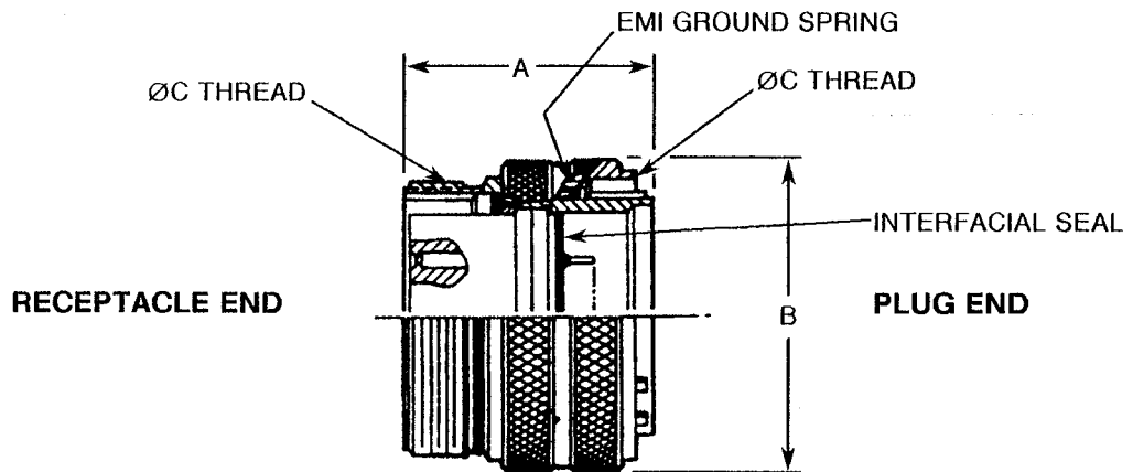
TYPE VARIANT 03 - SAVERS FOR 3401/056 CONNECTORS (SERIES III)
