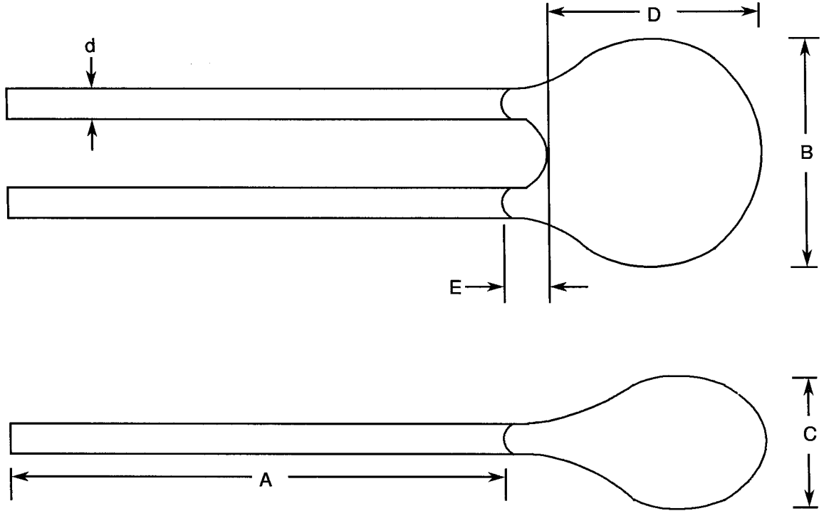
FIGURE 2 - PHYSICAL DIMENSIONS
