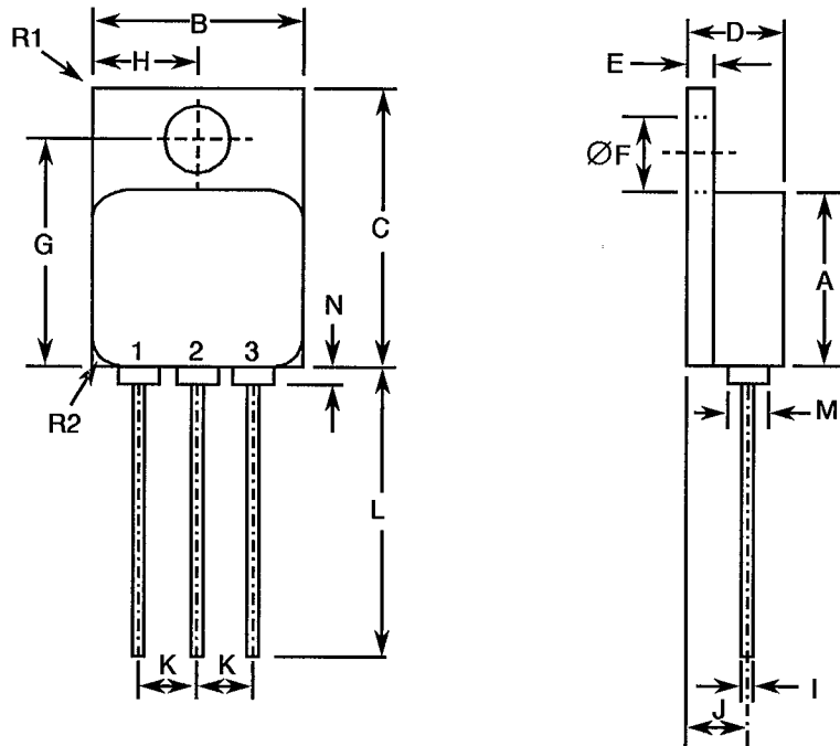
FIGURE 2 - PHYSICAL DIMENSIONS
