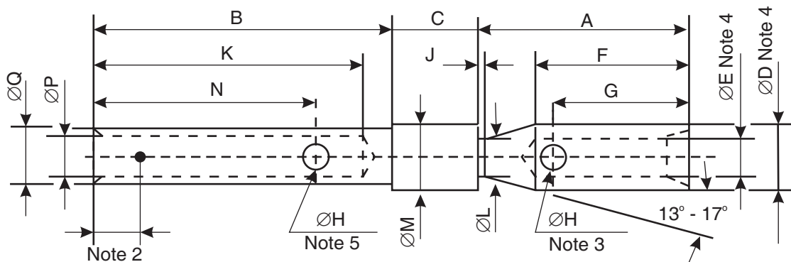
Figure 2.2 - Female Contact
