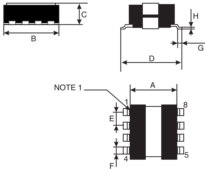
Figure 2 - PHYSICAL DIMENSIONS
