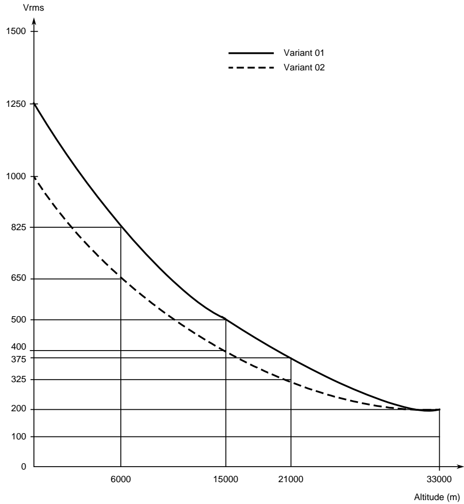
Voltage Proof versus Altitude
