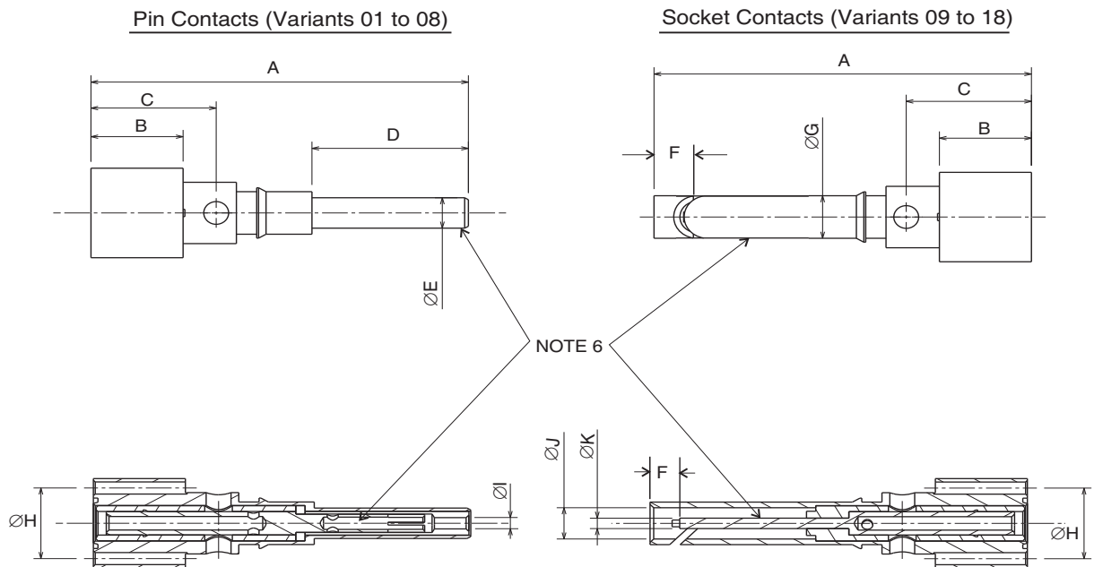
Figure 2(f) - Inner Contacts
