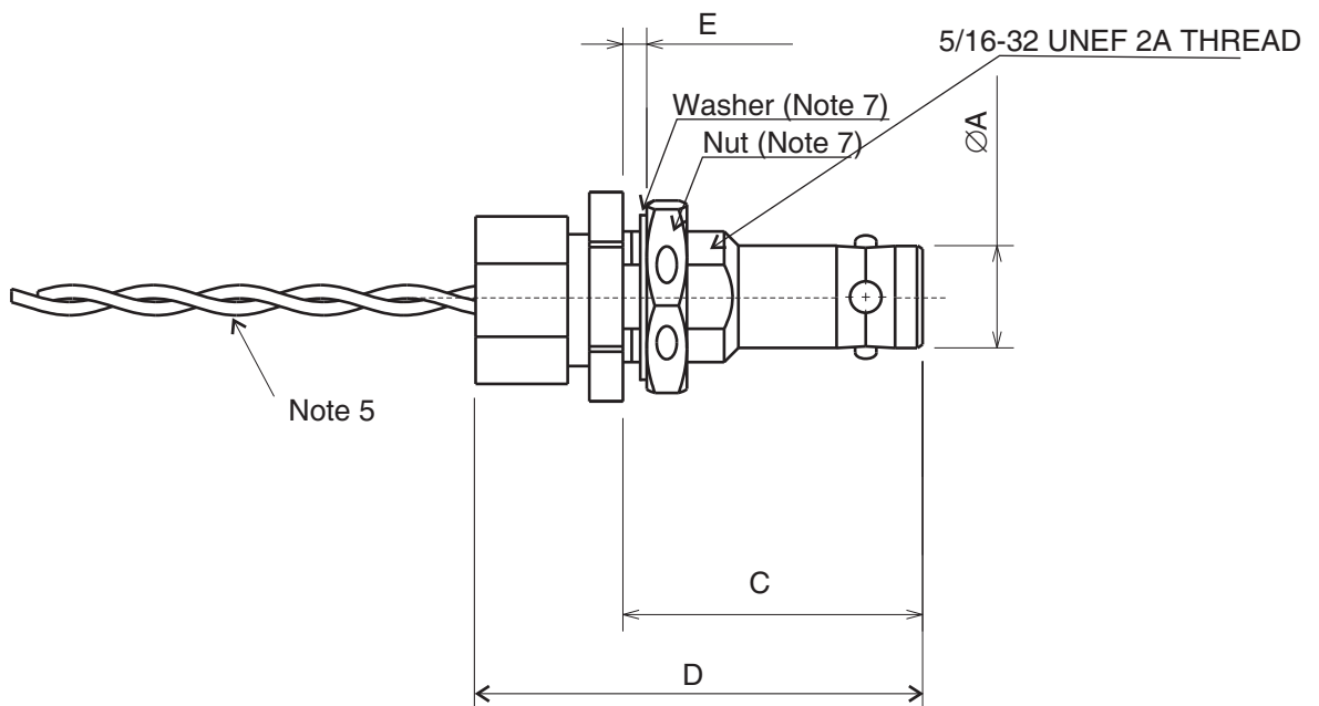
Figure 2(e) - Bulkhead Jack, Pigtail (Variants 17 and 18)
