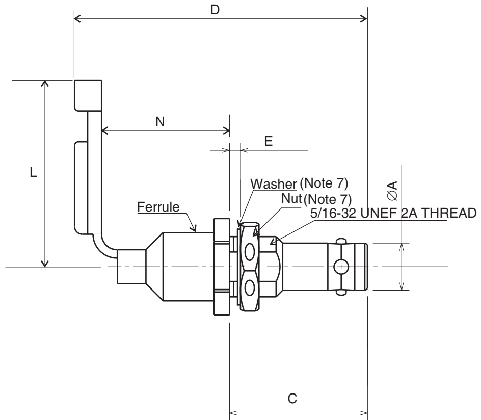
Figure 2(d) - Bulkhead Jack, Right Angle (Variants 11, 12, 15 and 16)
