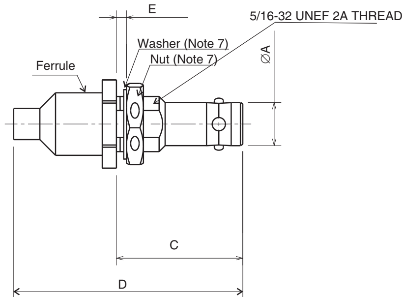
Figure 2(c) - Bulkhead Jack, Straight (Variants 09, 10, 13 and 14)
