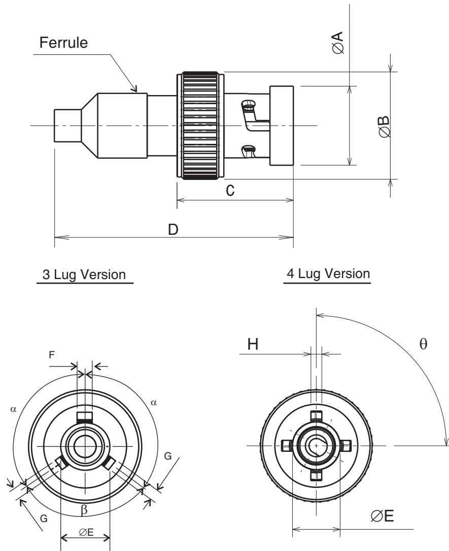
FIGURE 2(a) - Plug, Straight (Variants 01, 02, 05 and 06)
