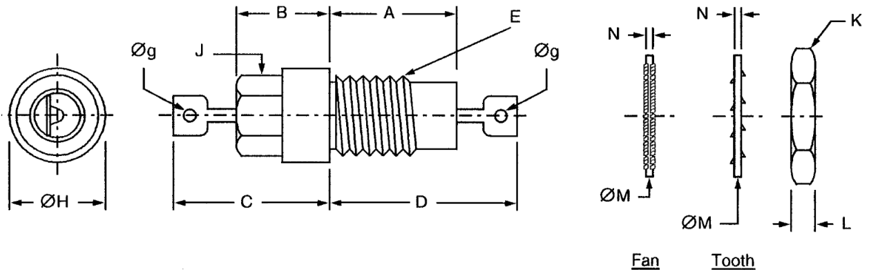
FIGURE 2 - PHYSICAL DIMENSIONS
