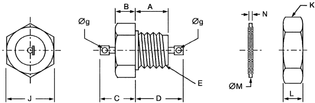
FIGURE 2 – PHYSICAL DIMENSIONS
