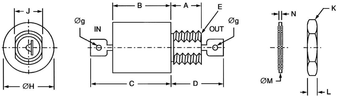
FIGURE 2 – PHYSICAL DIMENSIONS
