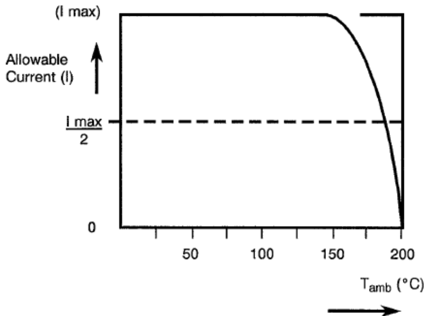
Allowable Current versus Temperature
