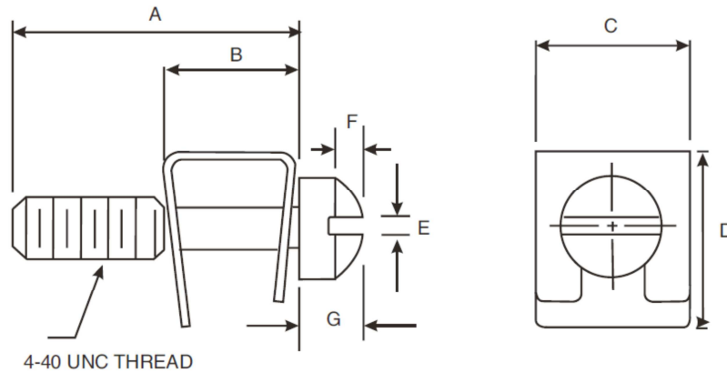
FIGURE 2(I) – MALE SCREW LOCK ASSEMBLY SLOTTED HEAD
