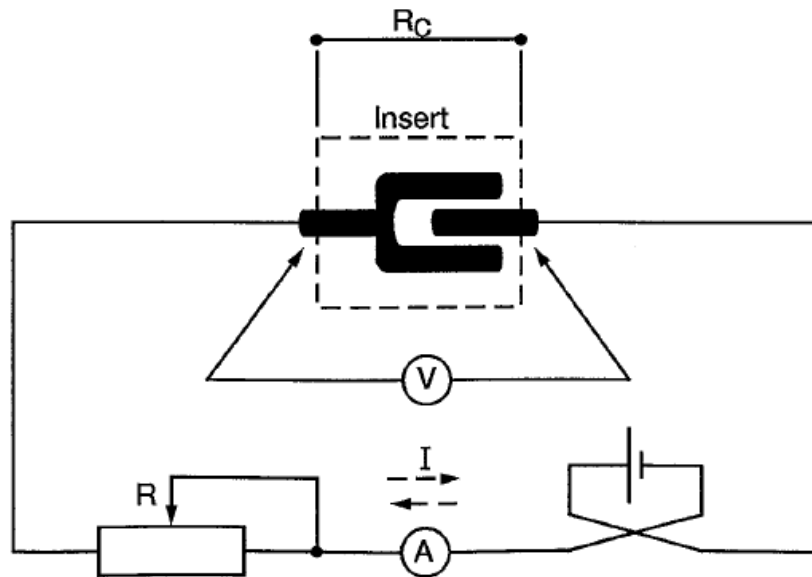
FIGURE I - CONTACT RESISTANCE MEASUREMENT DIAGRAM
