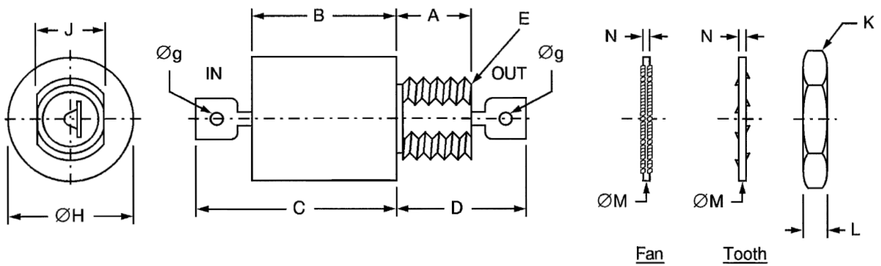
FIGURE 2 - PHYSICAL DIMENSIONS
