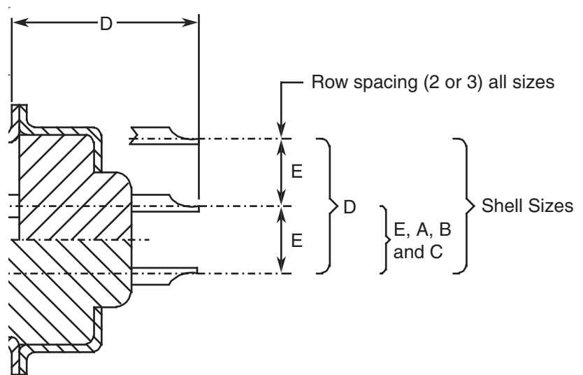
FIGURE 2(c) REAR END Gauge 20 Solder Bucket Contacts (CODE -)
