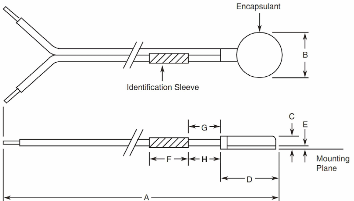
FIGURE 2 - PHYSICAL DIMENSIONS
