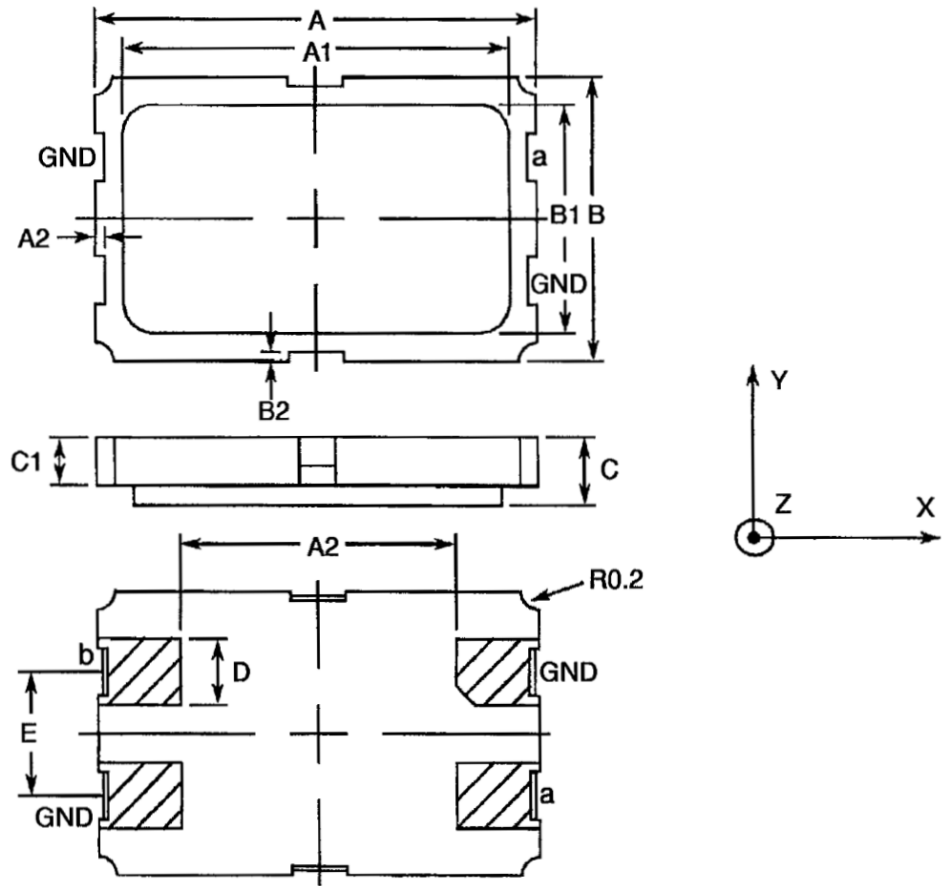
FIGURE 2 - PHYSICAL DIMENSIONS
