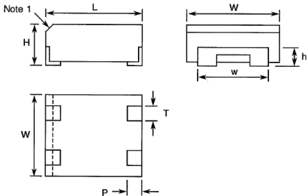
FIGURE 2 - PHYSICAL DIMENSIONS
