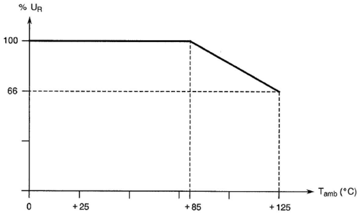
FIGURE 1(b) - RATED VOLTAGE VERSUS TEMPERATURE
