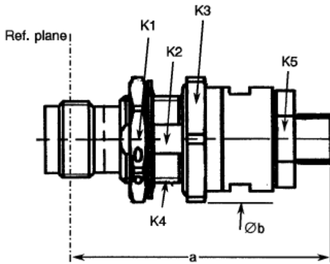
VARIANT 04 – STRAIGHT BULKHEAD JACK, SOLDER TYPE, FOR CABLE SHF 5
