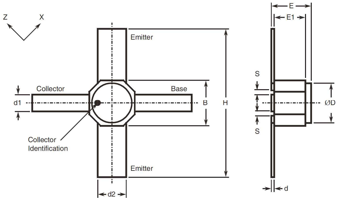
FIGURE 2 - PHYSICAL DIMENSIONS AND TERMINAL IDENTIFICATION
