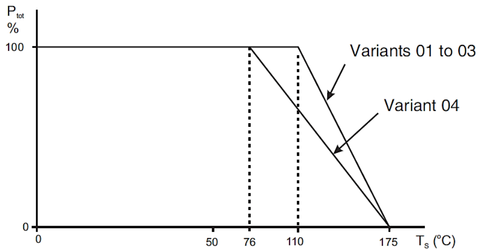
Power Dissipation versus Solder-Point Temperature
