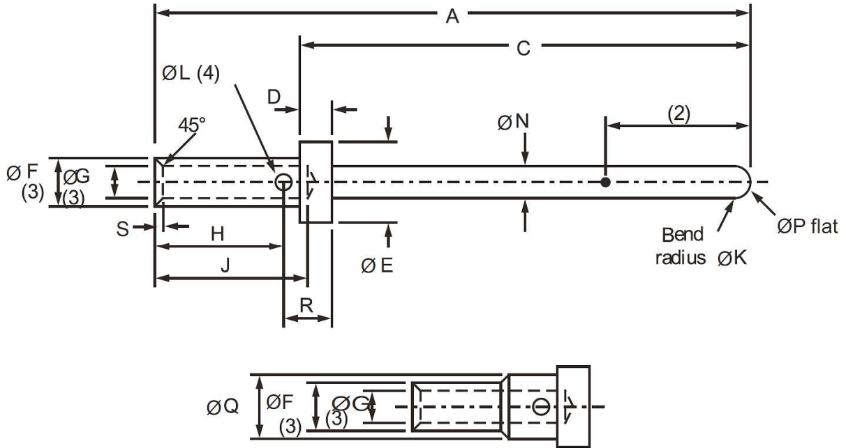
FIGURE 2 – PHYSICAL DIMENSIONS
