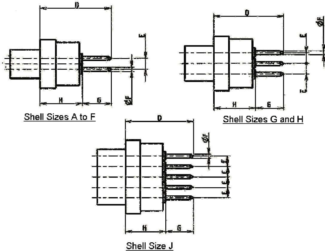
FIGURE 2(c) - REAR END
