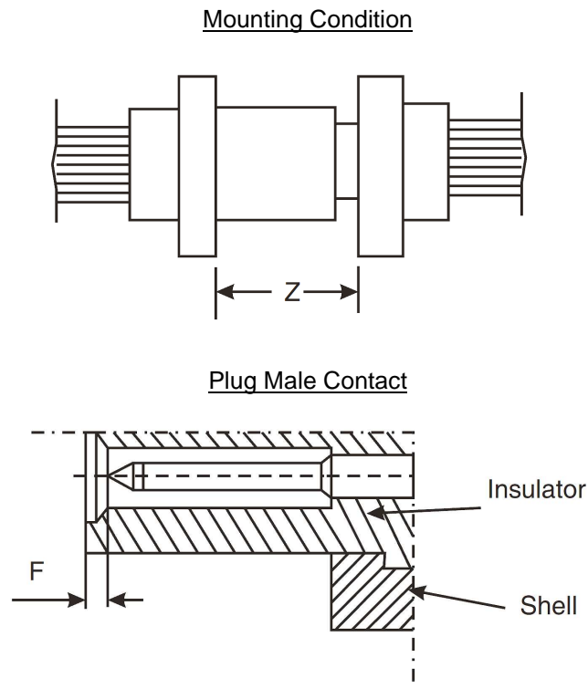
FIGURE 2(d) - MATING DIMENSIONS AND CONTACT POSITION
