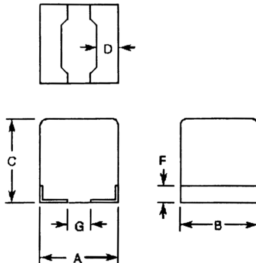
FIGURE 2 - PHYSICAL DIMENSIONS
