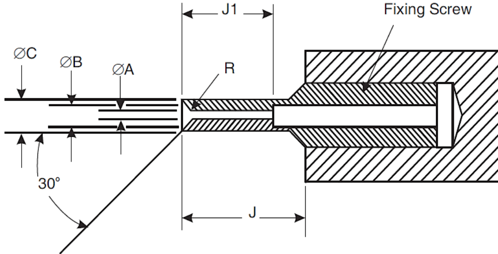
FIGURE 3 - GAUGE FIXTURE
